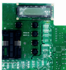
SPM014 Scheda GH2 display bianco GH2 board with white display
